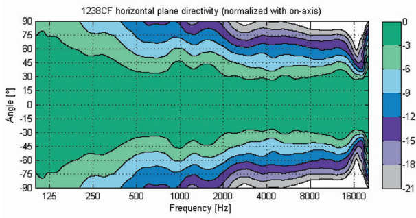
Figure 10. Horizontal directivity characteristics of the 1238DF.
