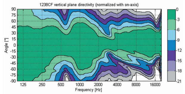
Figure 11. Vertical directivity characteristics of the 1238DF.
