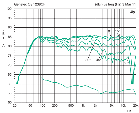
Figure 12. Horizontal directivity characteristics of the 1238DF. The lower curve is the monitor's power response.
